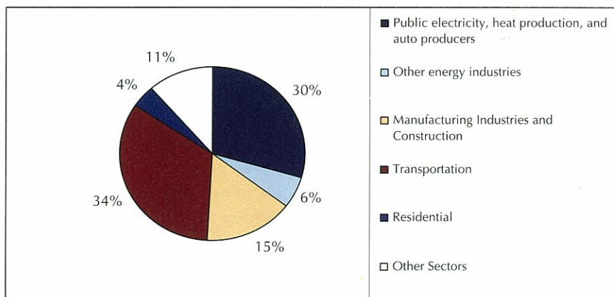
Sectoral CO 2 emissions (1999) Source: World Resource Institute 2003
