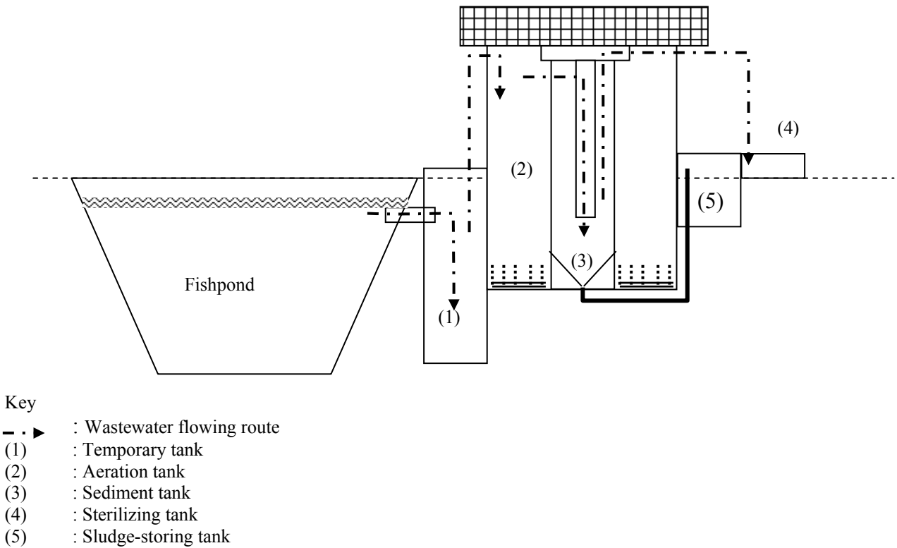
Figure 1. Aeration svstem
