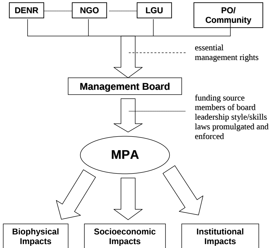
Figure 1. Analytical Framework
