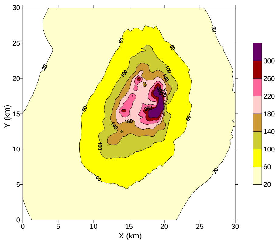
Figure 6. Isoline map of average annual concentration ( \mu\text{g}/\text{m}^3 ) of \text{SO}_2 with IGCC in Guiyang
