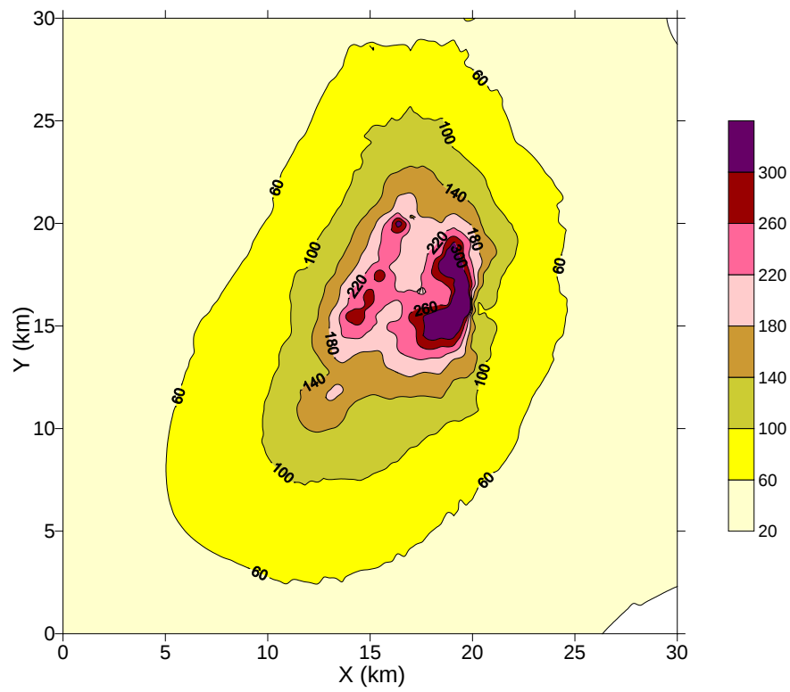
Figure 4. Isoline map of average annual concentration ( \mu\text{g}/\text{m}^3 ) of SO 2 in the baseline scenario in Guiyang
