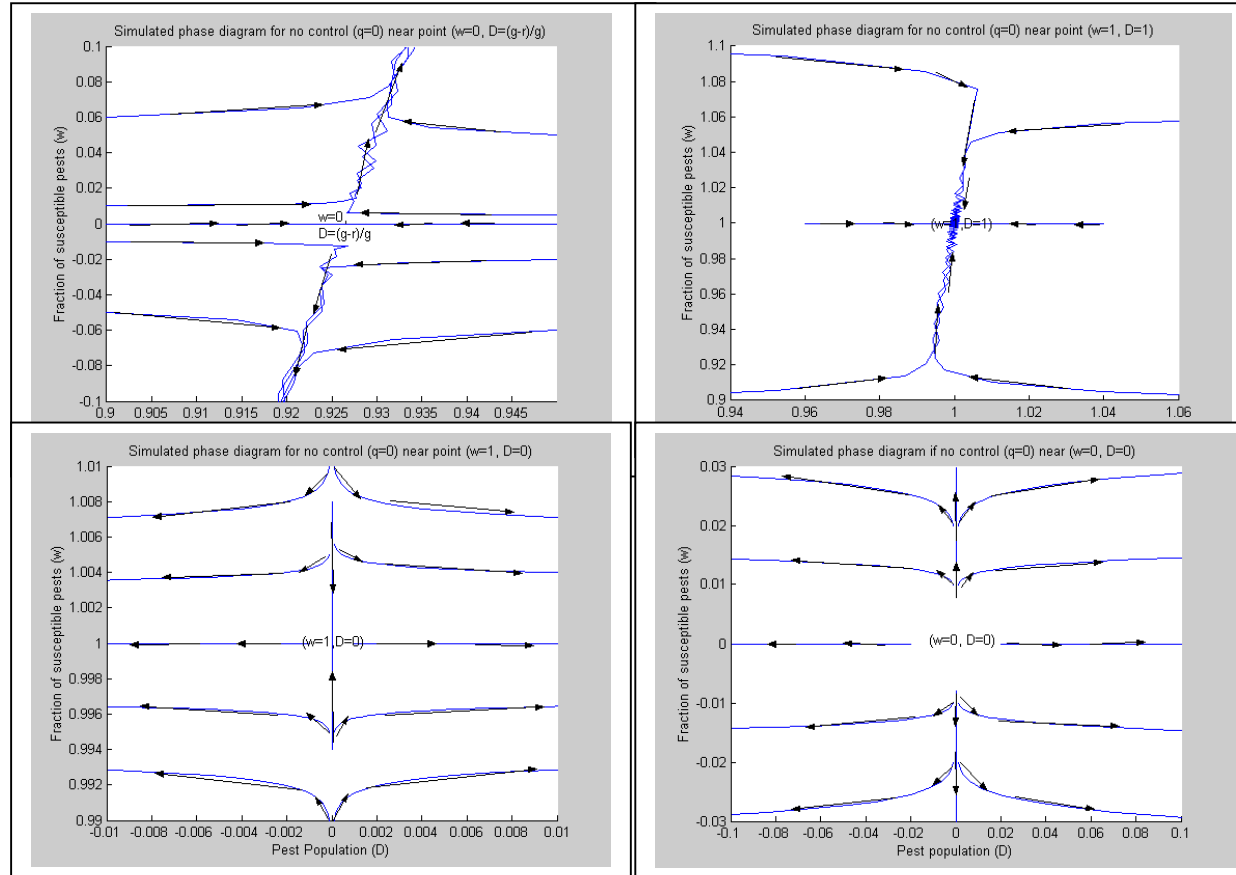
Figure 2-A3. Numerical analysis of the characteristics of the four fixed points led by the no control strategy: ( D=0, w=0 ) and ( D=0, w=1 ) are two saddle points, ( D=1, w=1 ) is an asymptotically stable node while ( D=\frac{g-r}{g}, w=0 ) is an unstable star node.
