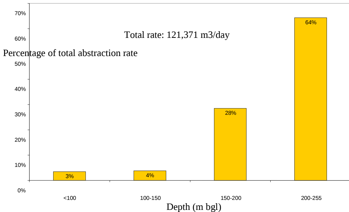
Figure 6. COWD wells: depth and abstraction rate, May 2010
